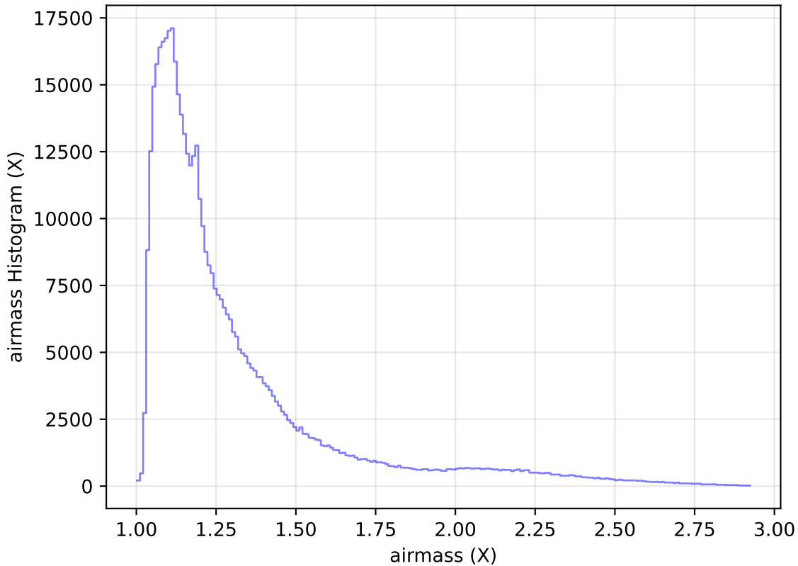
internal_u_expt38_nscale0.9v3.4_10yrs All sky i band: airmass Histogram
