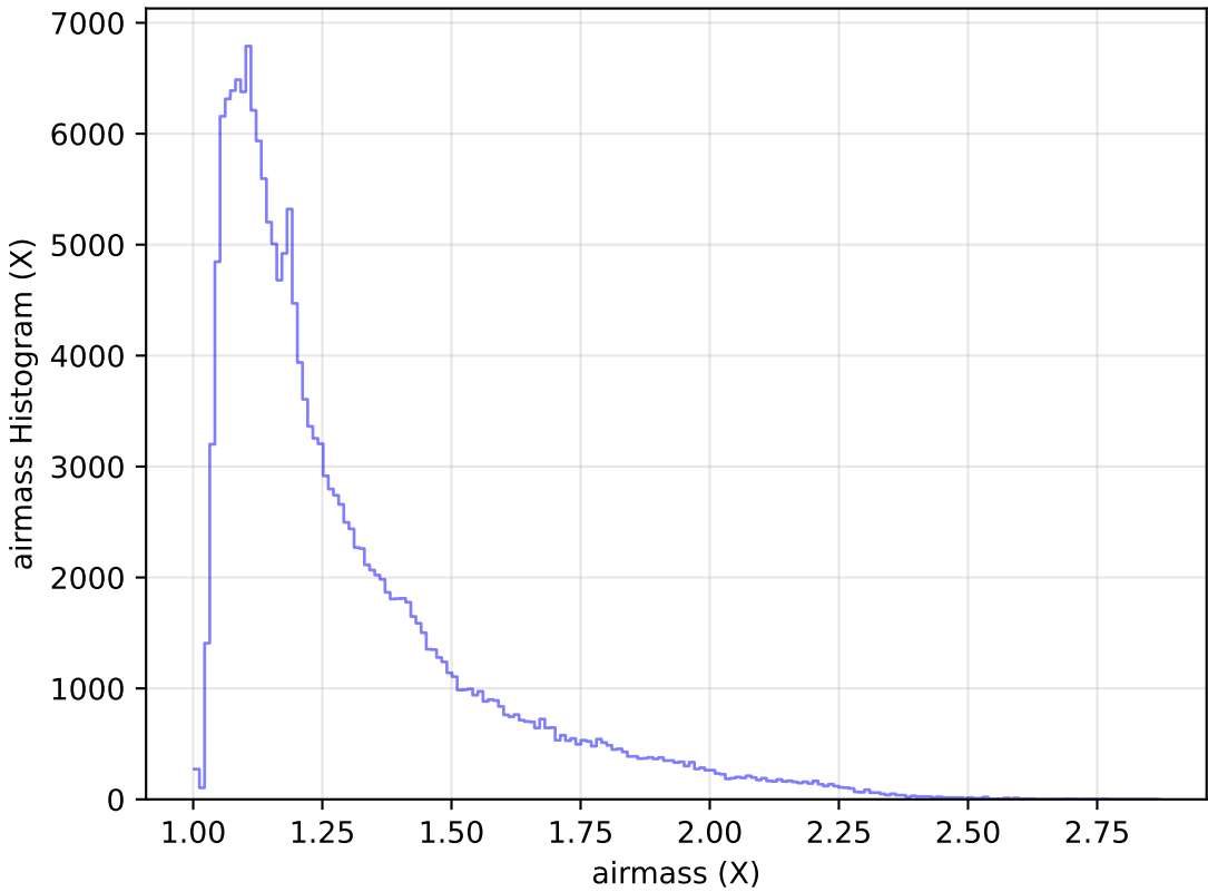
internal_u_expt38_nscale0.9v3.4_10yrs All sky g band: airmass Histogram
