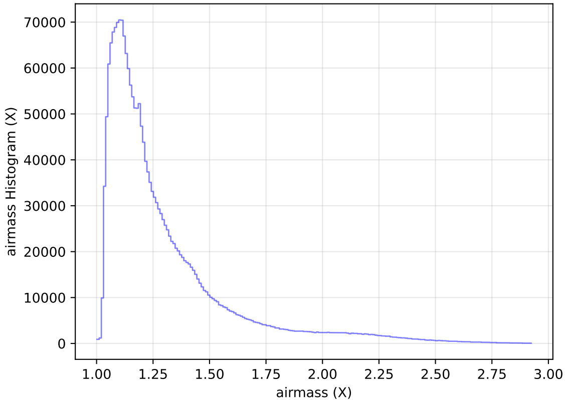
internal_u_expt38_nscale0.9v3.4_10yrs All sky all bands: airmass Histogram
