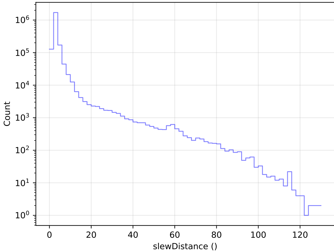
internal_u_expt38_nscale0.9v3.4_10yrs All visits: Slew Distance Histogram
