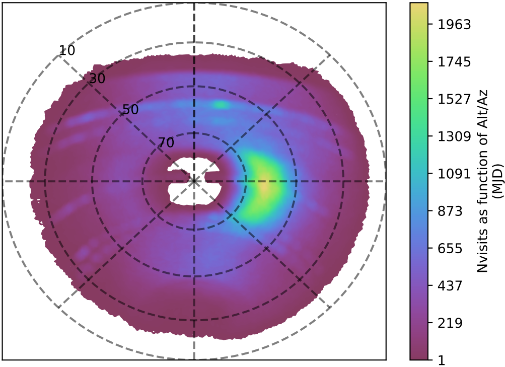
internal_u_expt38_nscale0.9v3.4_10yrs y band: Nvisits as function of Alt/Az
