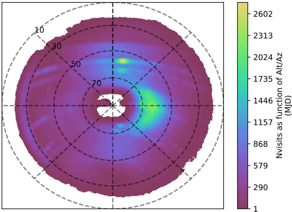
internal_u_expt38_nscale0.9v3.4_10yrs r band: Nvisits as function of Alt/Az
