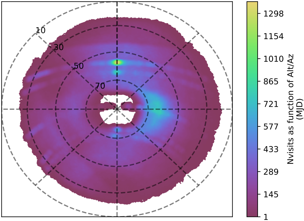
internal_u_expt38_nscale0.9v3.4_10yrs g band: Nvisits as function of Alt/Az
