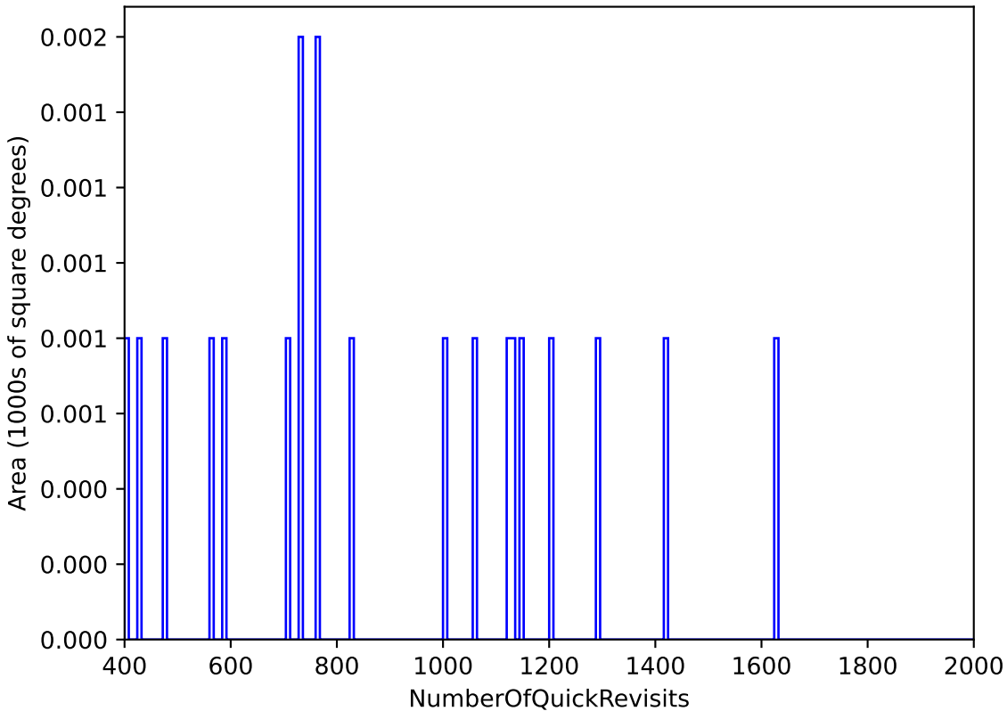
internal_u_expt38_nscale0.9v3.4_10yrs WFD: NumberOfQuickRevisits
