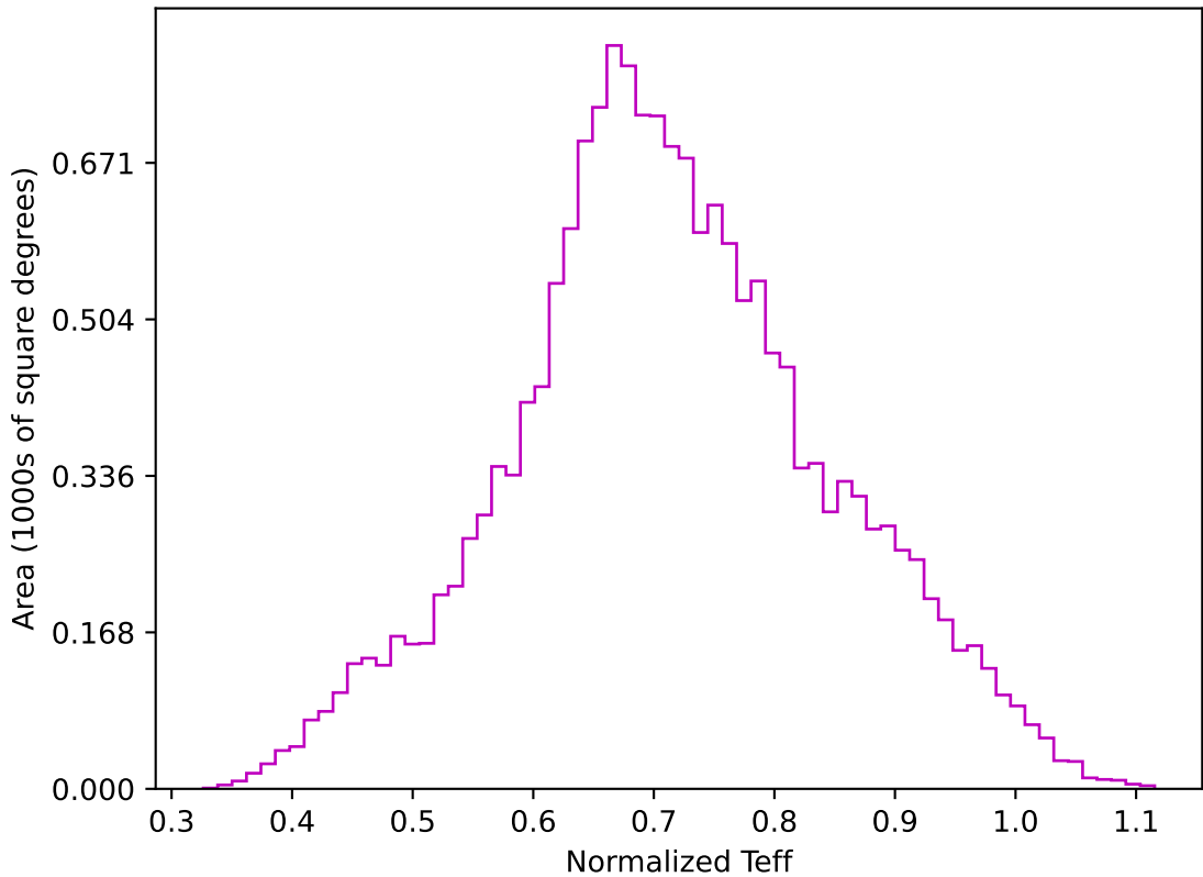
internal_u_expt38_nscale0.9v3.4_10yrs WFD z band: Normalized Teff
