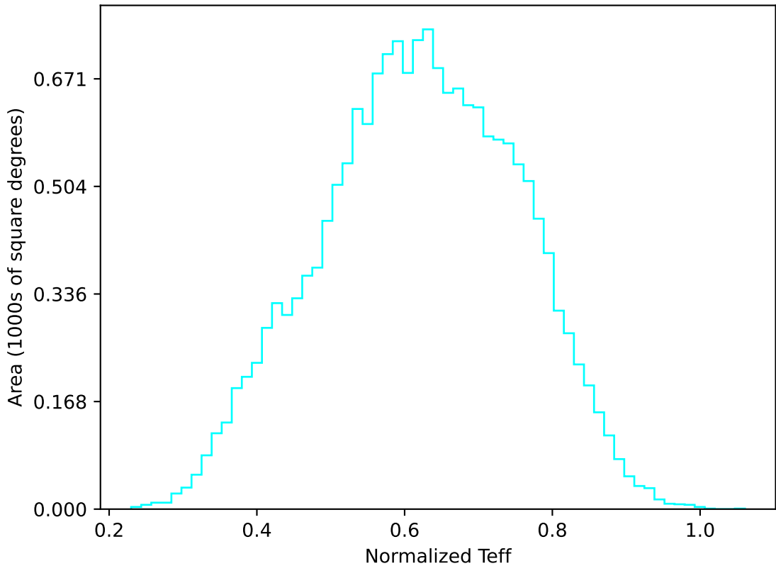
internal_u_expt38_nscale0.9v3.4_10yrs WFD u band: Normalized Teff
