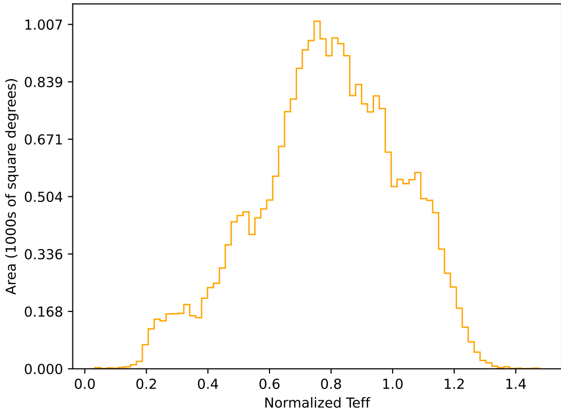
internal_u_expt38_nscale0.9v3.4_10yrs All sky r band: Normalized Teff
