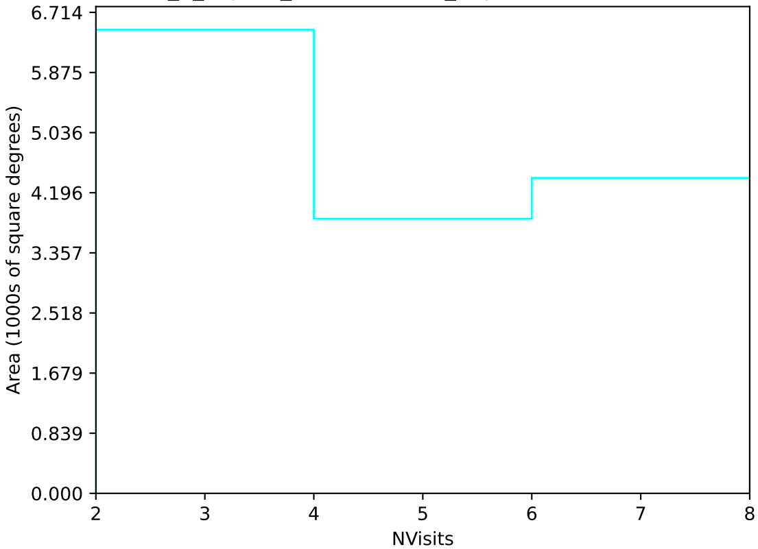
internal_u_expt38_nscale0.9v3.4_10yrs Yr 3-4 u band: NVisits
