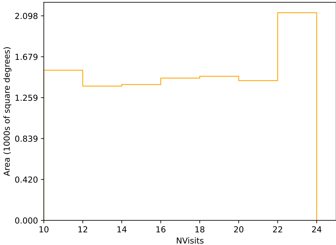
internal_u_expt38_nscale0.9v3.4_10yrs Yr 3-4 r band: NVisits
