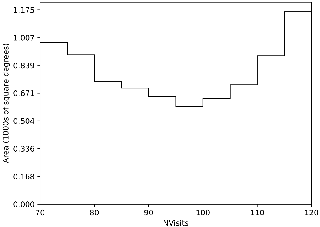
internal_u_expt38_nscale0.9v3.4_10yrs Yr 3-4 all bands: NVisits
