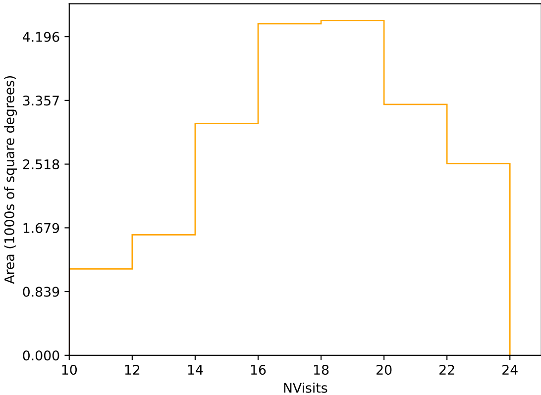
internal_u_expt38_nscale0.9v3.4_10yrs Yr 1 r band: NVisits
