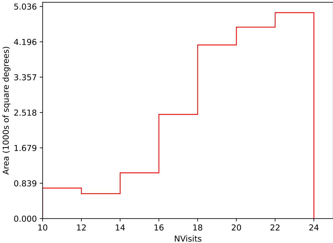
internal_u_expt38_nscale0.9v3.4_10yrs Yr 1 i band: NVisits
