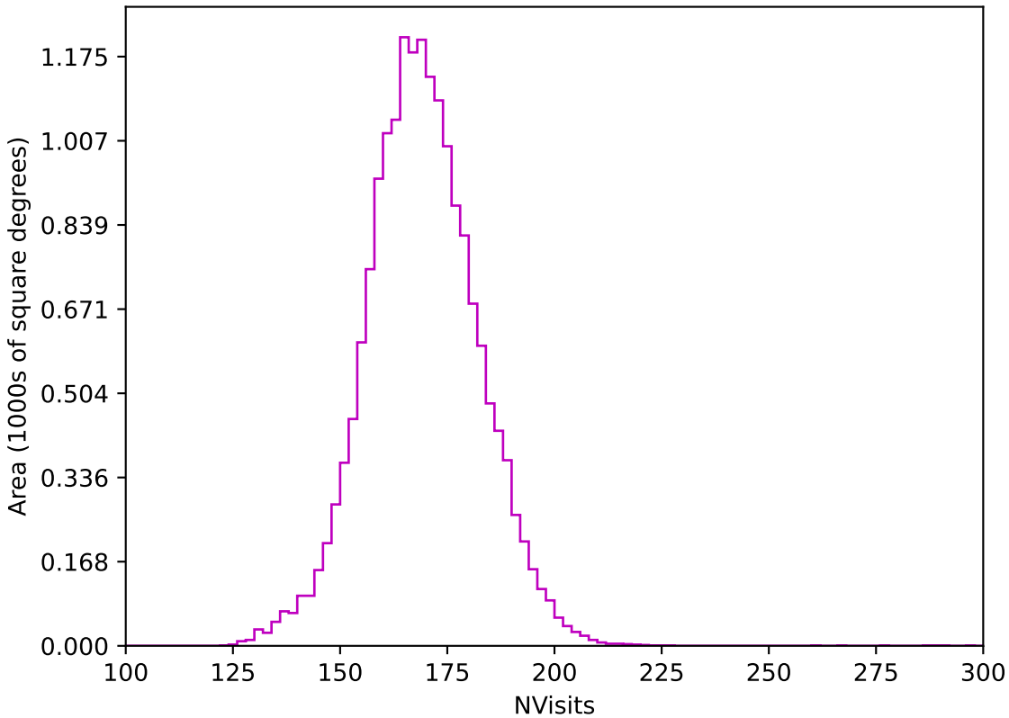
internal_u_expt38_nscale0.9v3.4_10yrs WFD z band: NVisits
