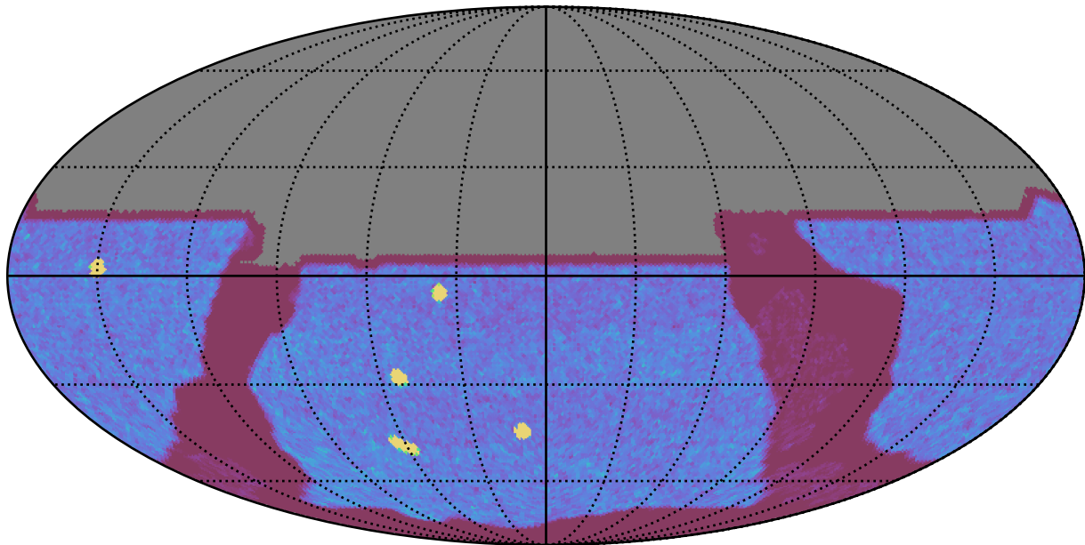
internal_u_expt38_nscale0.9v3.4_10yrs All sky y band: NVisits
