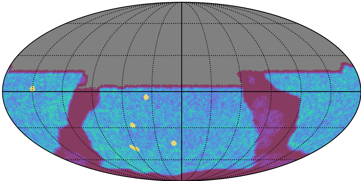
internal_u_expt38_nscale0.9v3.4_10yrs All sky u band: NVisits
