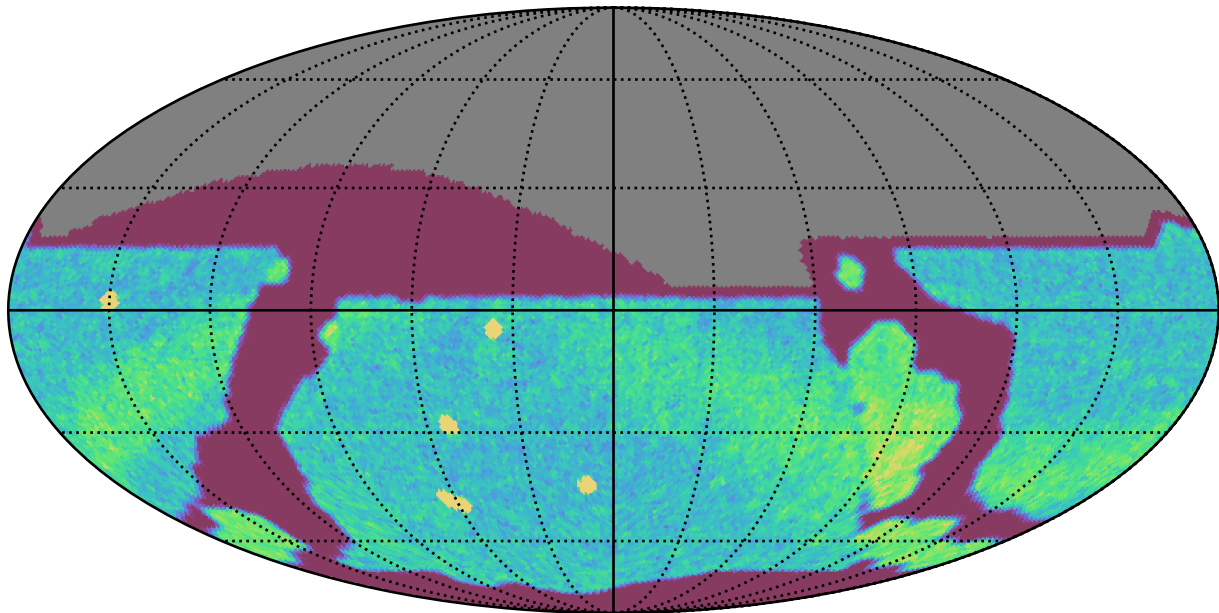
internal_u_expt38_nscale0.9v3.4_10yrs All sky r band: NVisits
