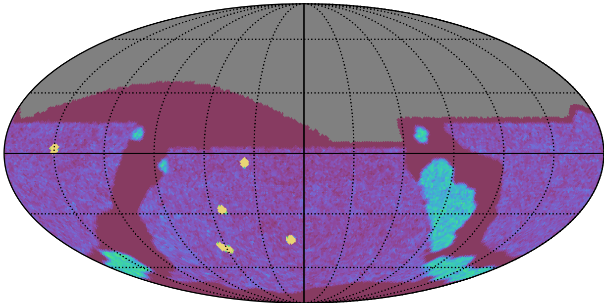
internal_u_expt38_nscale0.9v3.4_10yrs All sky g band: NVisits
