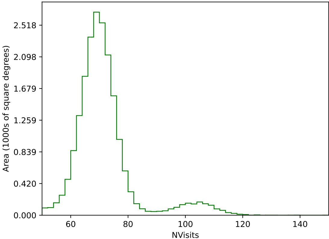
internal_u_expt38_nscale0.9v3.4_10yrs All sky g band: NVisits
