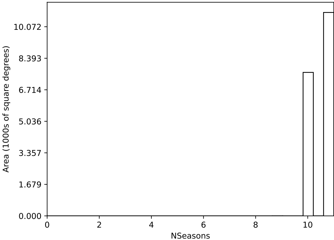
internal_u_expt38_nscale0.9v3.4_10yrs WFD all bands: NSeasons
