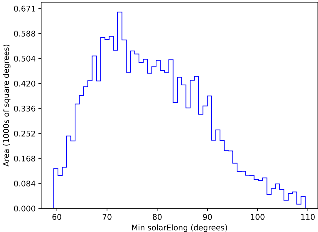
internal_u_expt38_nscale0.9v3.4_10yrs WFD u band: Min solarElong
