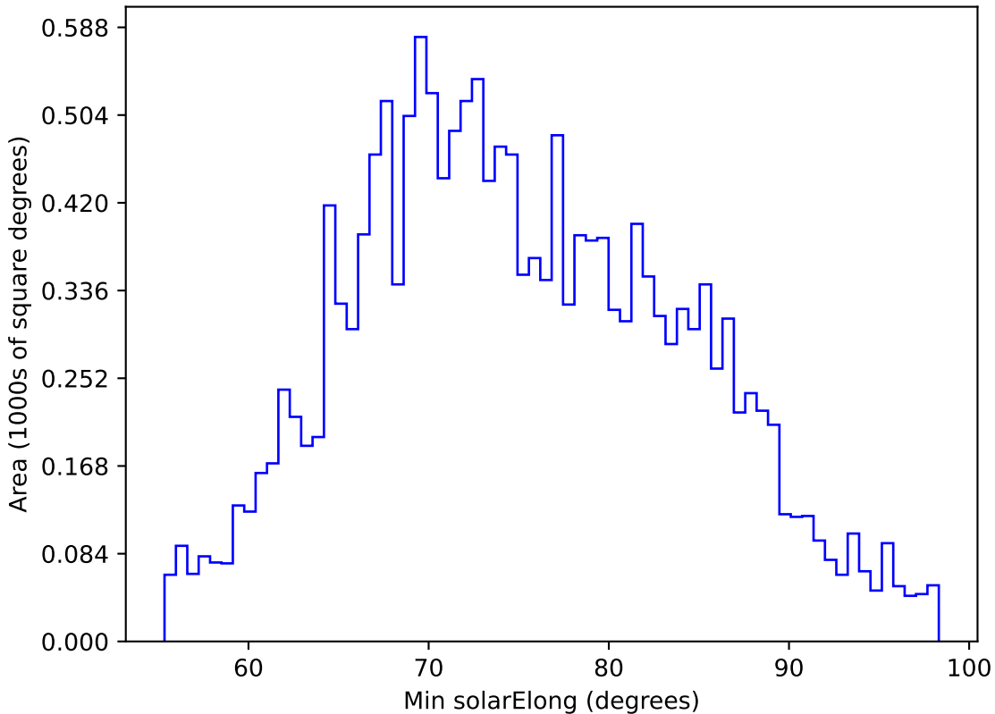
internal_u_expt38_nscale0.9v3.4_10yrs WFD g band: Min solarElong
