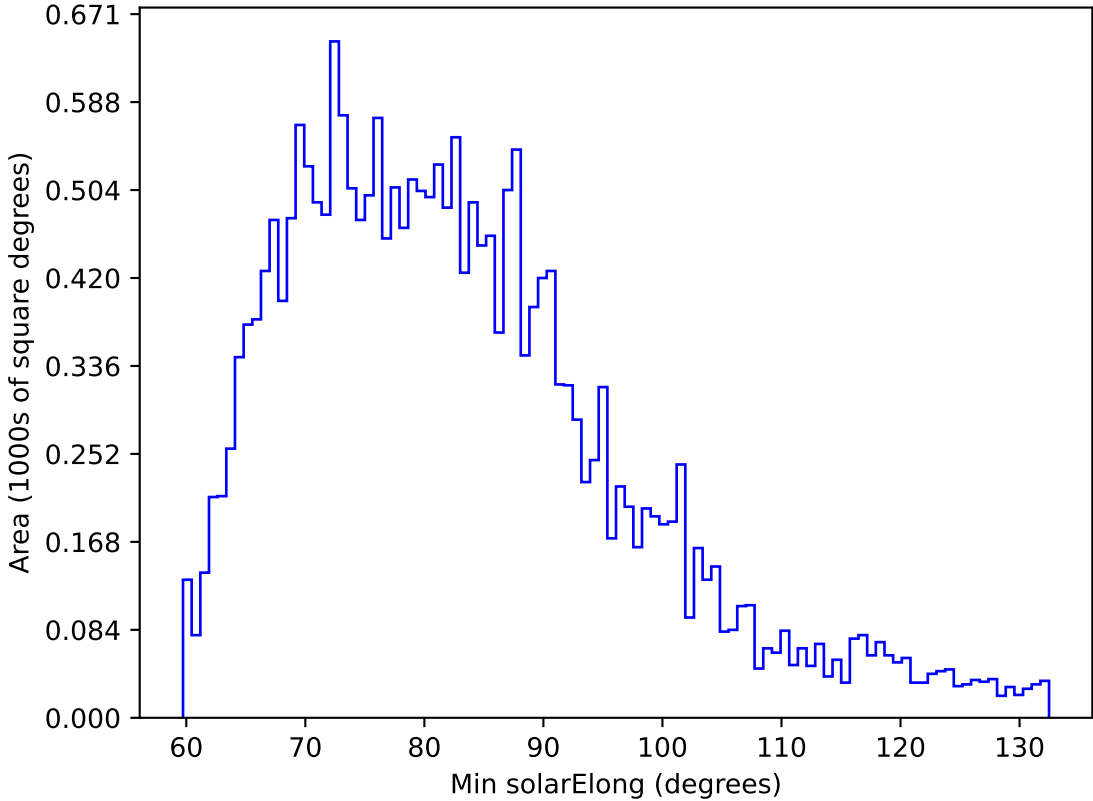
internal_u_expt38_nscale0.9v3.4_10yrs All sky u band: Min solarElong
