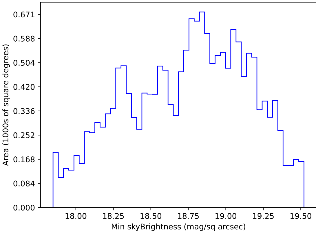
internal_u_expt38_nscale0.9v3.4_10yrs WFD r band: Min skyBrightness
