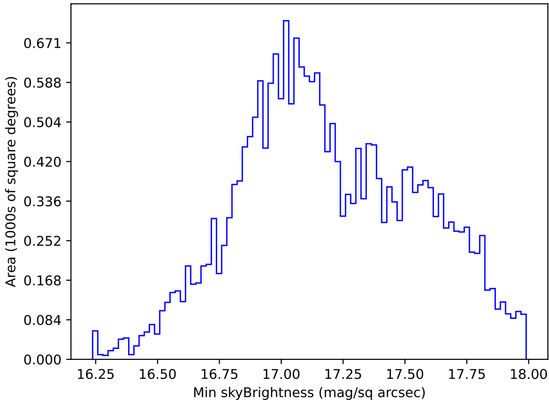
internal_u_expt38_nscale0.9v3.4_10yrs All sky y band: Min skyBrightness
