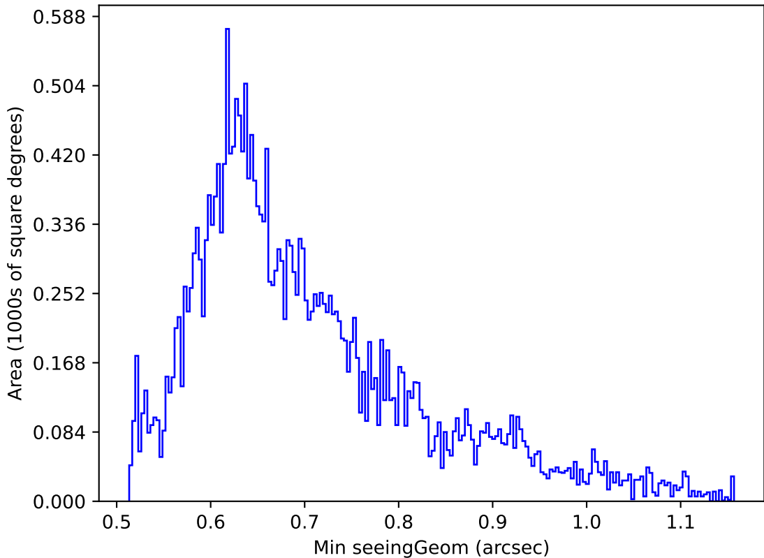
internal_u_expt38_nscale0.9v3.4_10yrs Yr 1 g band: Min seeingGeom
