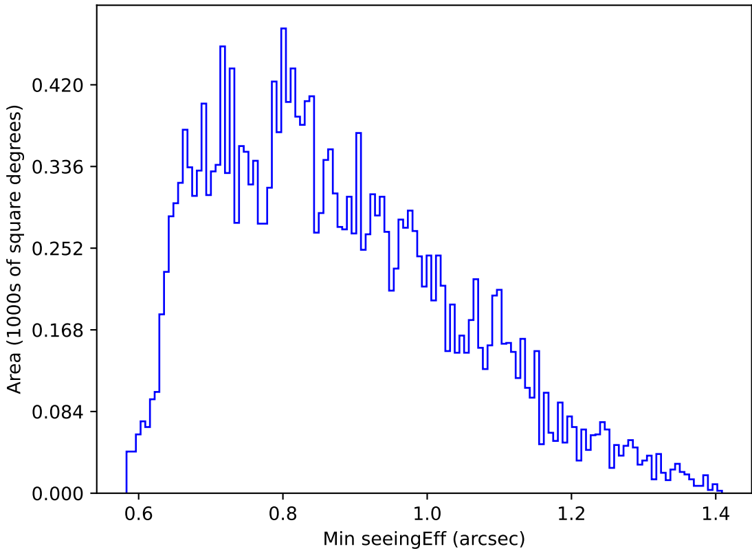
internal_u_expt38_nscale0.9v3.4_10yrs Yr 1 u band: Min seeingEff
