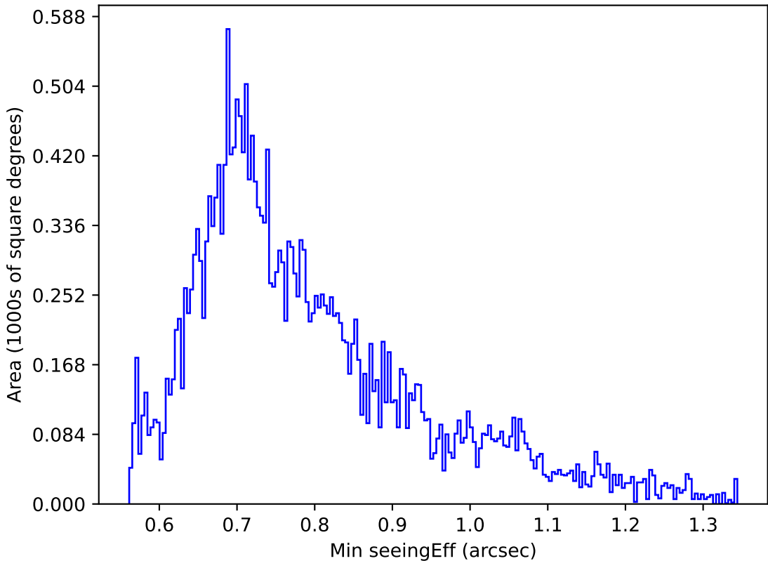
internal_u_expt38_nscale0.9v3.4_10yrs Yr 1 g band: Min seeingEff
