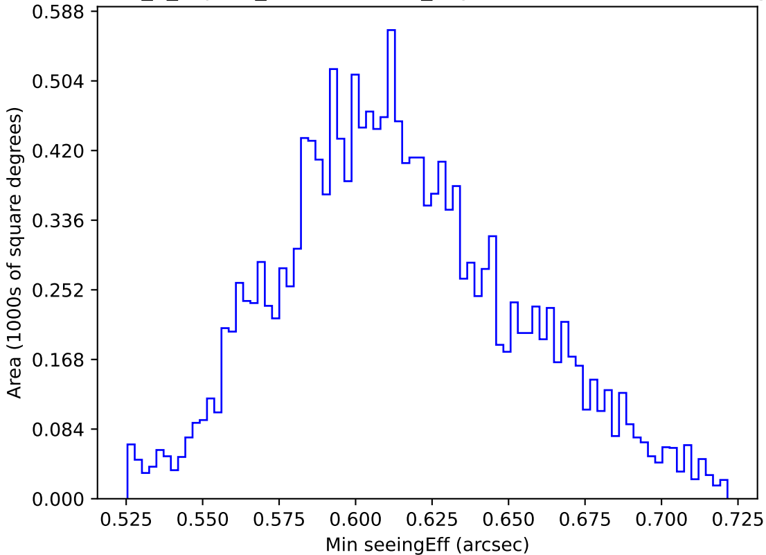
internal_u_expt38_nscale0.9v3.4_10yrs WFD z band: Min seeingEff
