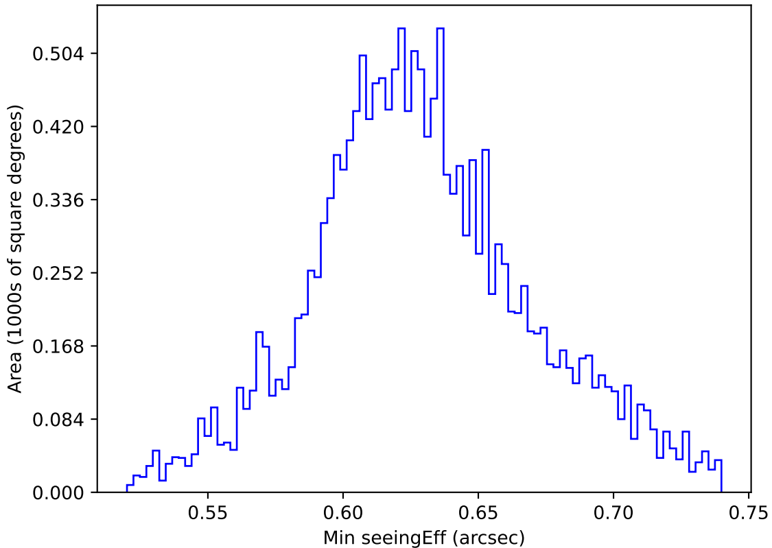
internal_u_expt38_nscale0.9v3.4_10yrs WFD y band: Min seeingEff
