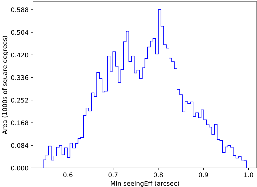
internal_u_expt38_nscale0.9v3.4_10yrs WFD u band: Min seeingEff
