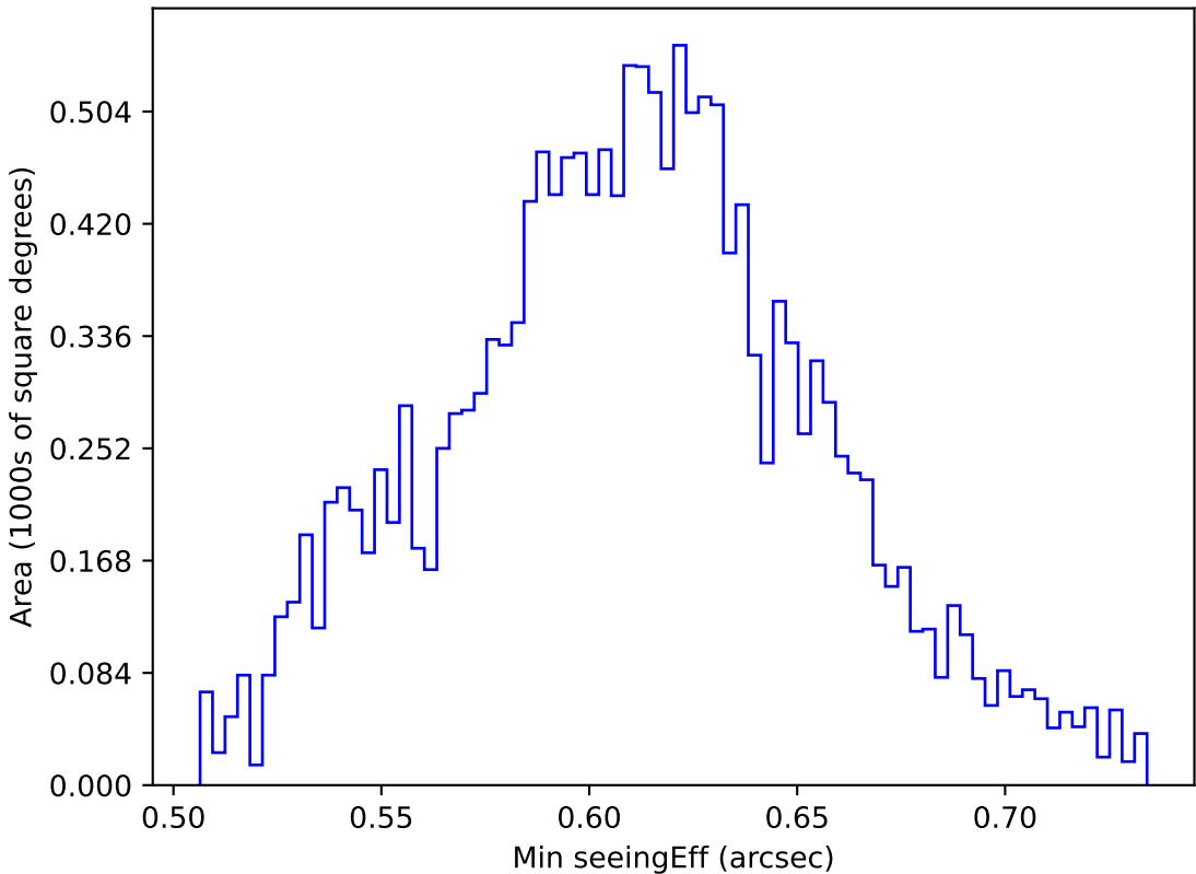
internal_u_expt38_nscale0.9v3.4_10yrs WFD r band: Min seeingEff
