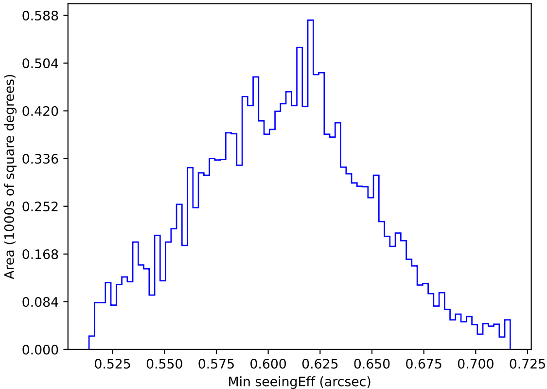
internal_u_expt38_nscale0.9v3.4_10yrs WFD i band: Min seeingEff
