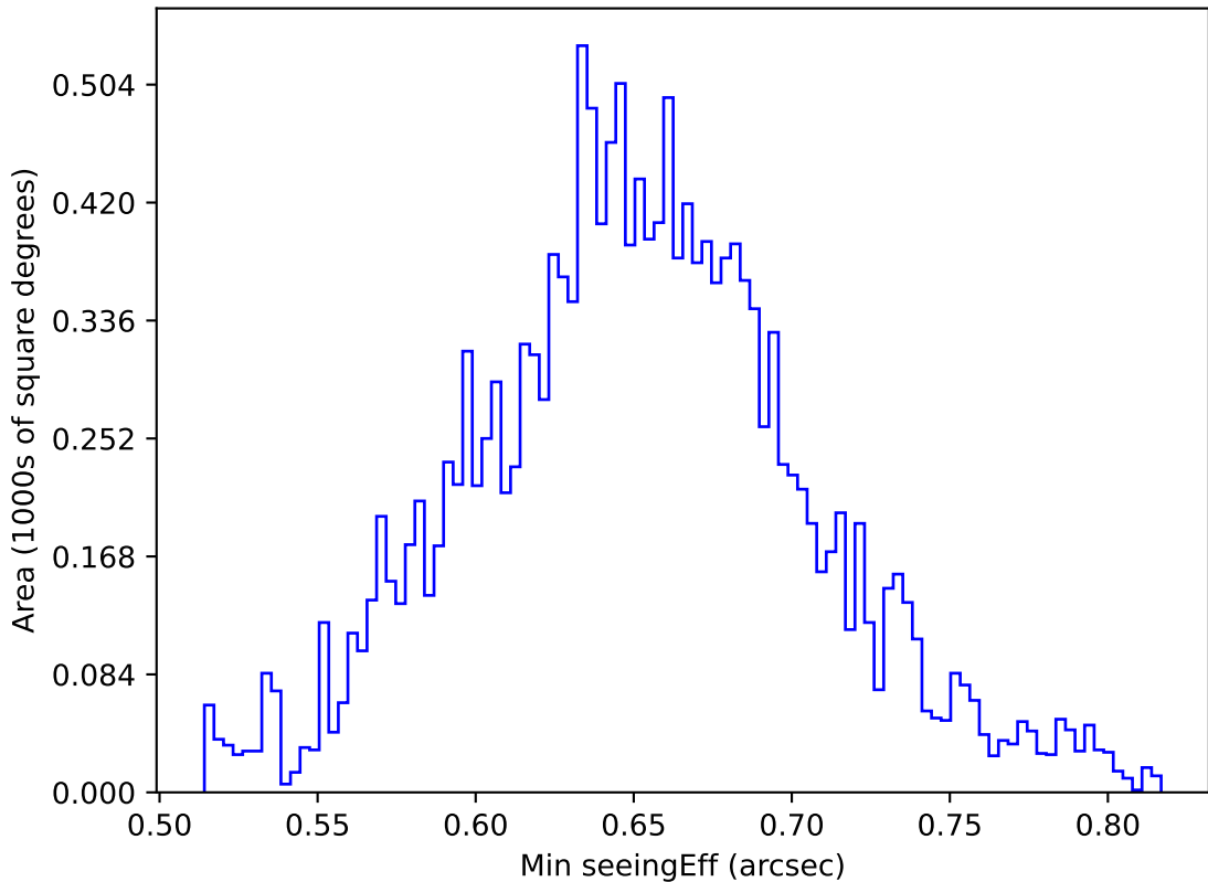
internal_u_expt38_nscale0.9v3.4_10yrs WFD g band: Min seeingEff
