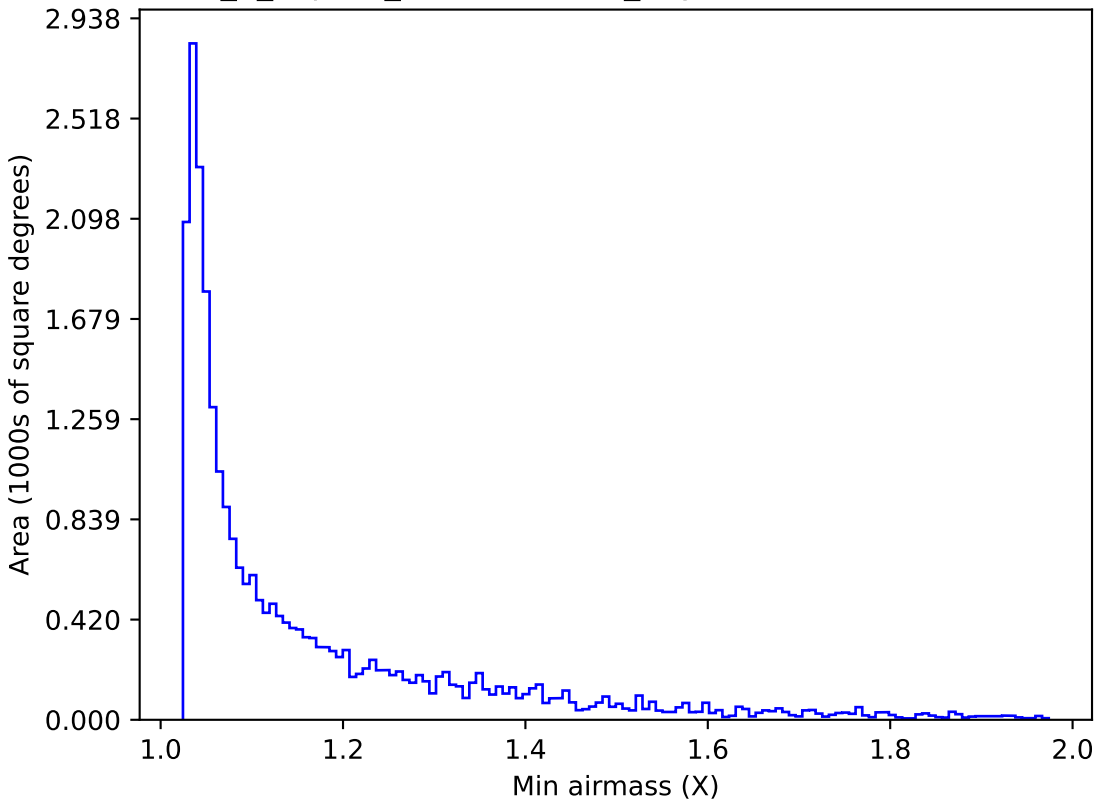
internal_u_expt38_nscale0.9v3.4_10yrs Yr 1 z band: Min airmass
