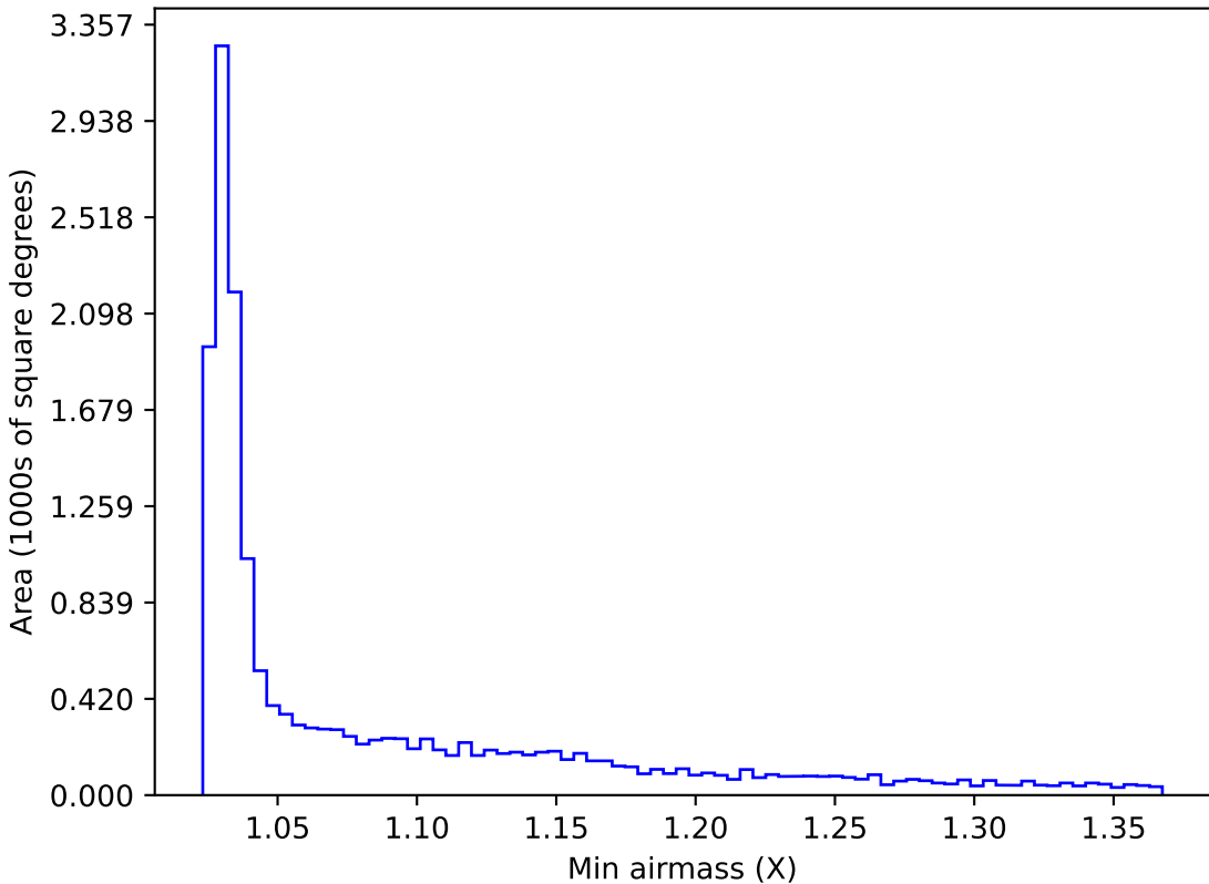
internal_u_expt38_nscale0.9v3.4_10yrs WFD y band: Min airmass
