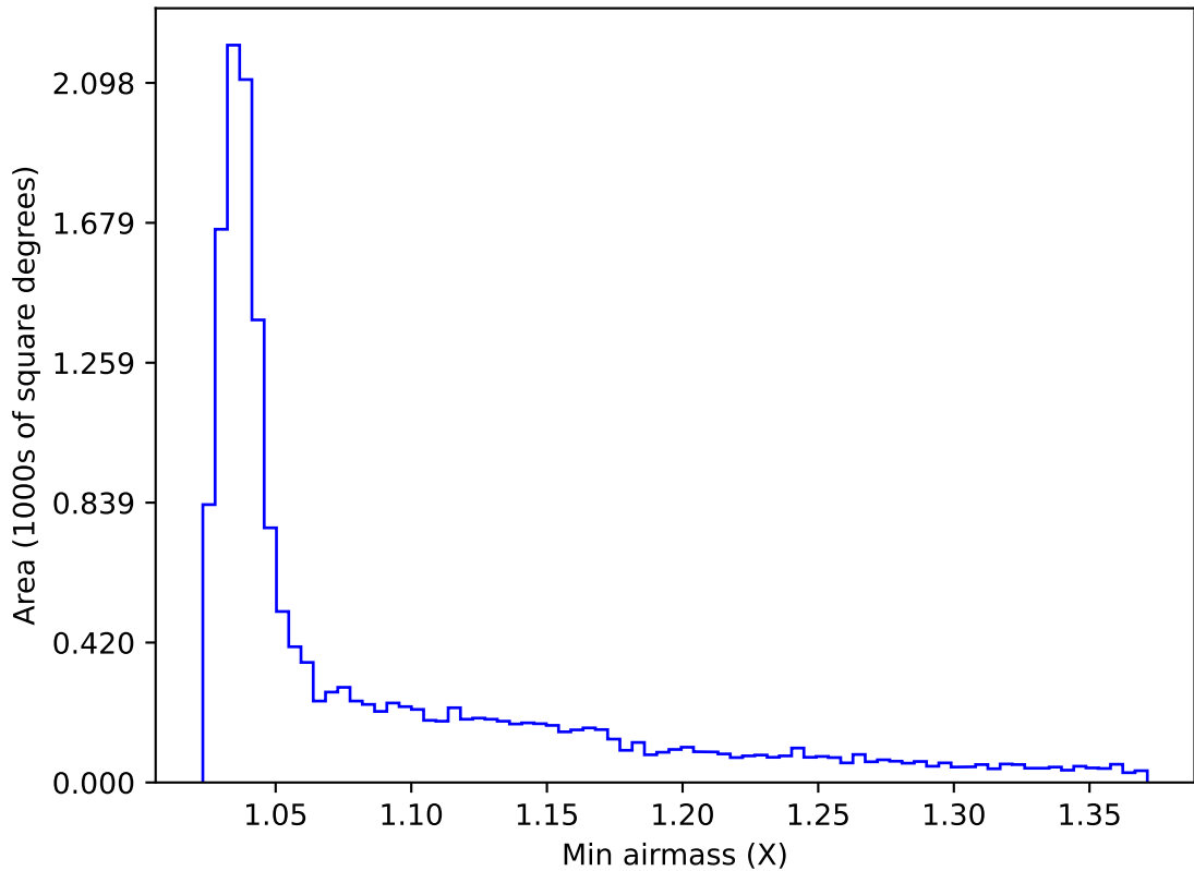
internal_u_expt38_nscale0.9v3.4_10yrs WFD g band: Min airmass
