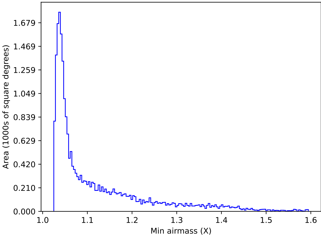
internal_u_expt38_nscale0.9v3.4_10yrs All sky u band: Min airmass
