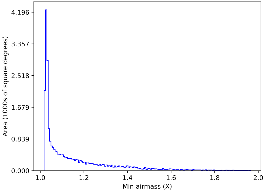
internal_u_expt38_nscale0.9v3.4_10yrs All sky r band: Min airmass
