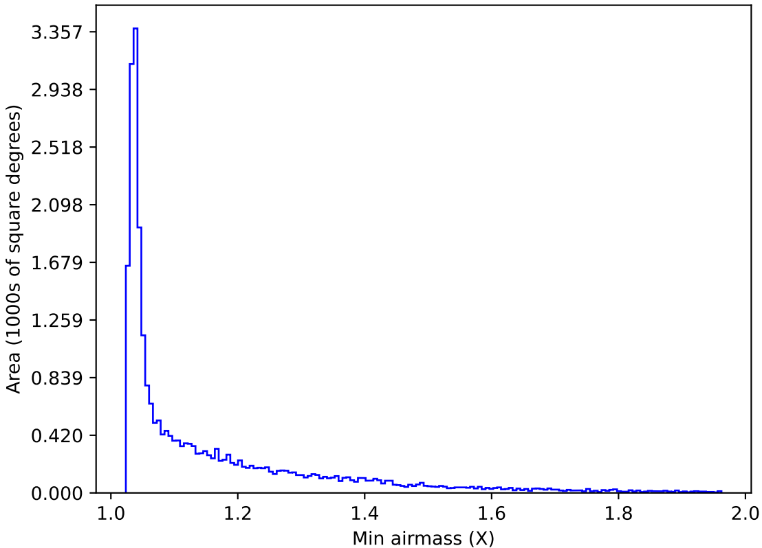
internal_u_expt38_nscale0.9v3.4_10yrs All sky g band: Min airmass
