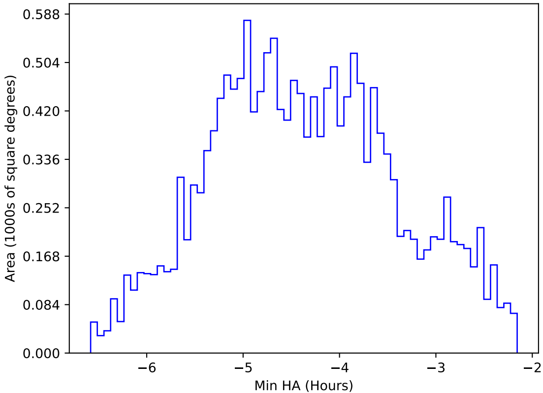
internal_u_expt38_nscale0.9v3.4_10yrs WFD z band: Min HA
