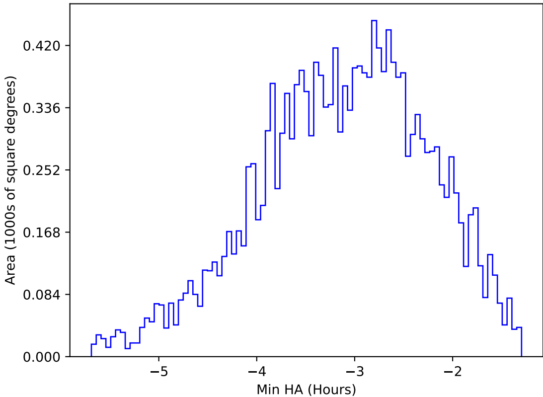
internal_u_expt38_nscale0.9v3.4_10yrs WFD u band: Min HA
