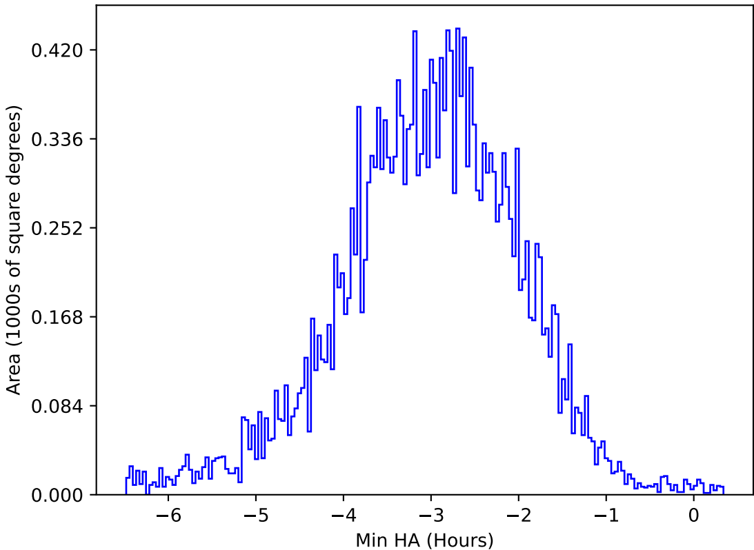
internal_u_expt38_nscale0.9v3.4_10yrs All sky u band: Min HA
