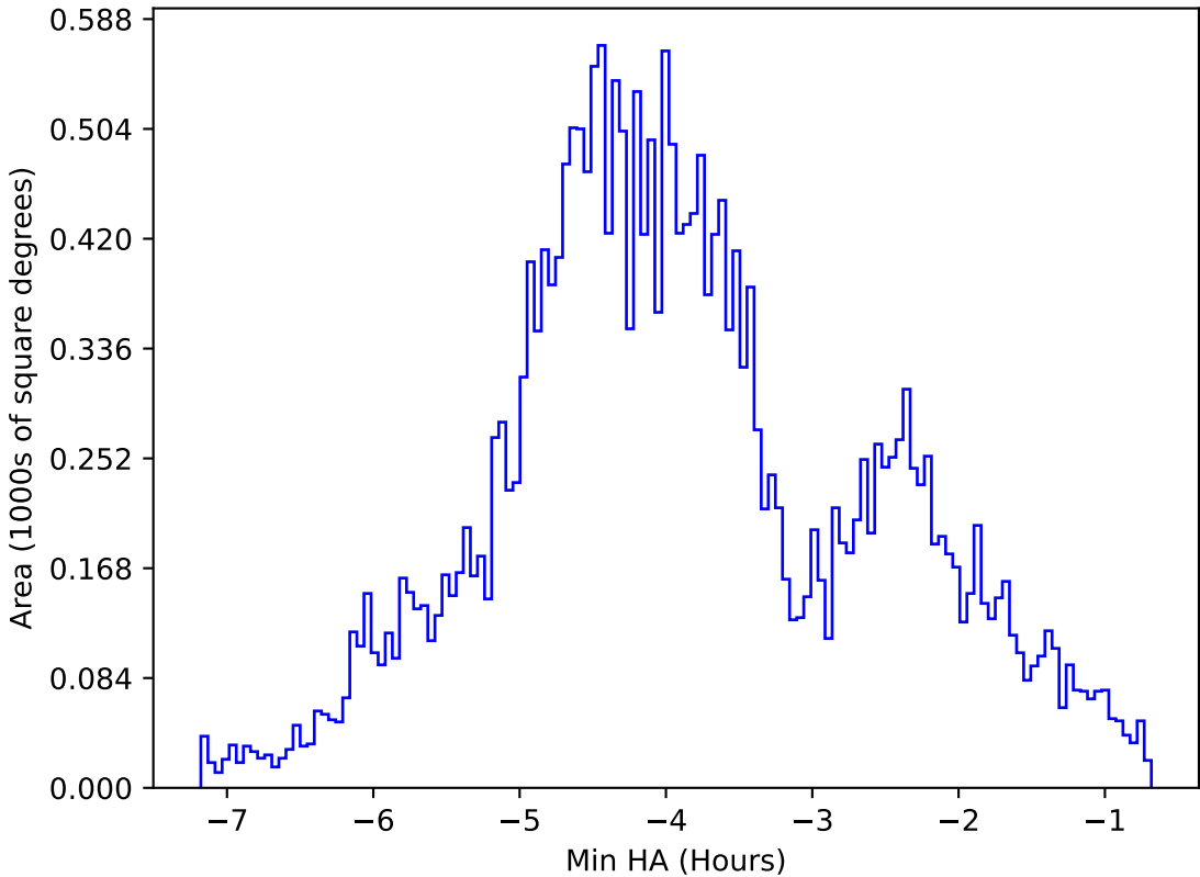
internal_u_expt38_nscale0.9v3.4_10yrs All sky g band: Min HA
