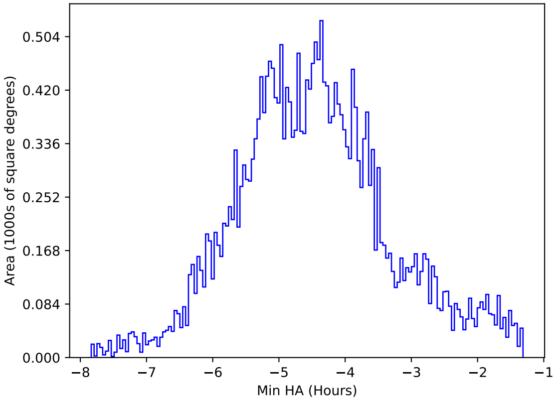
internal_u_expt38_nscale0.9v3.4_10yrs All sky all bands: Min HA
