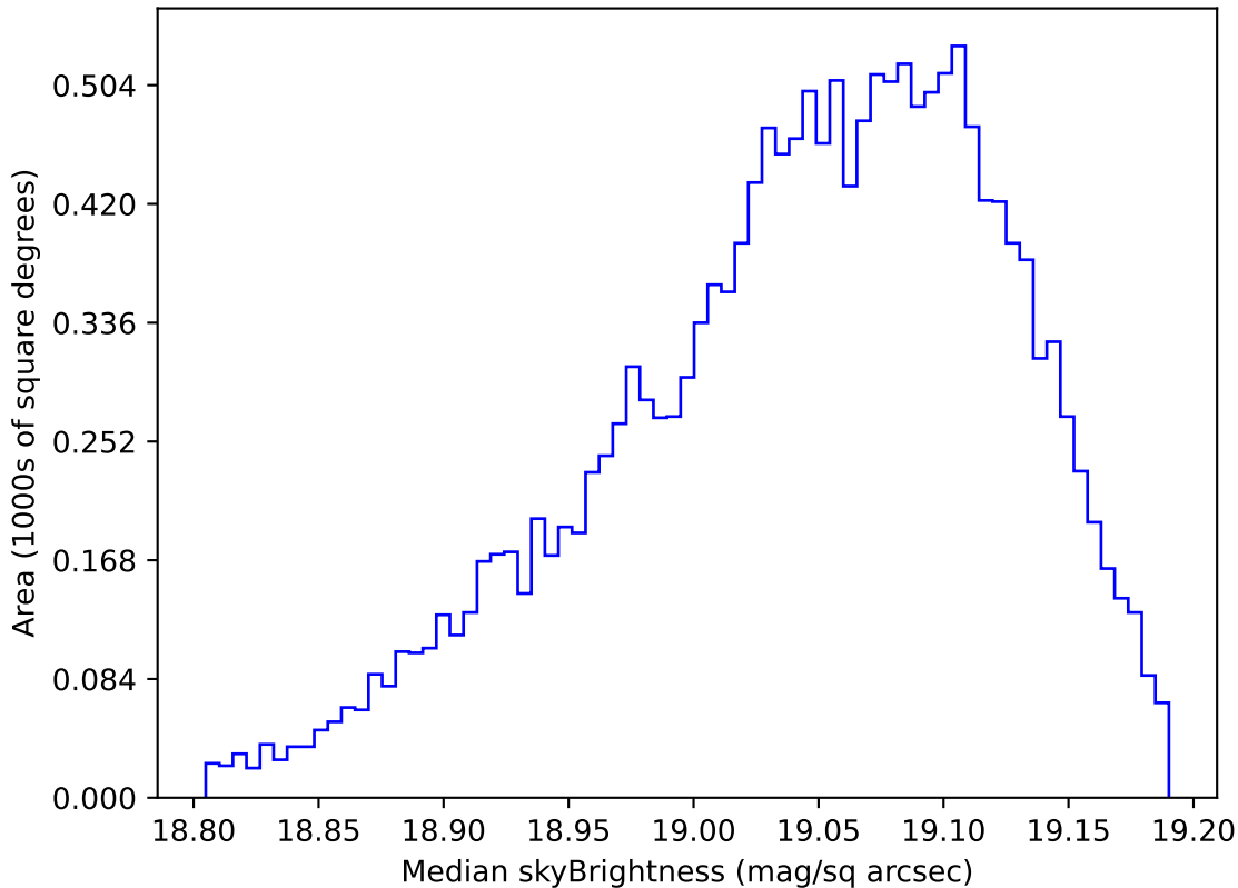
internal_u_expt38_nscale0.9v3.4_10yrs WFD z band: Median skyBrightness
