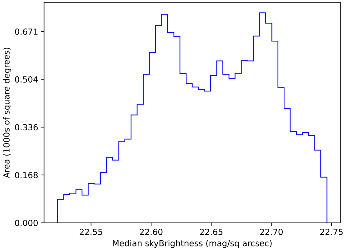
internal_u_expt38_nscale0.9v3.4_10yrs WFD u band: Median skyBrightness
